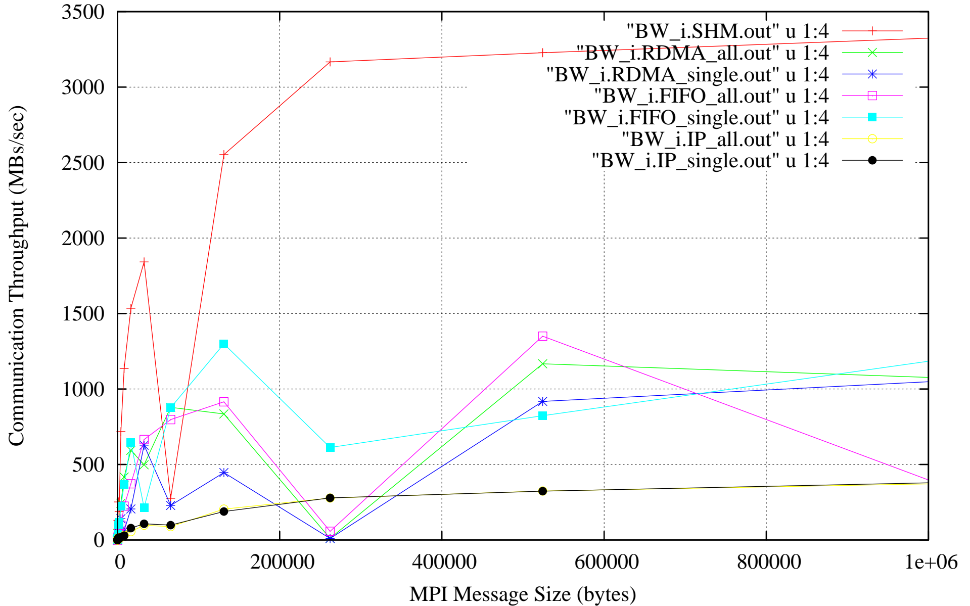
POE/MPI Communication Modes: Worst (shared, blocking, interrupts)
