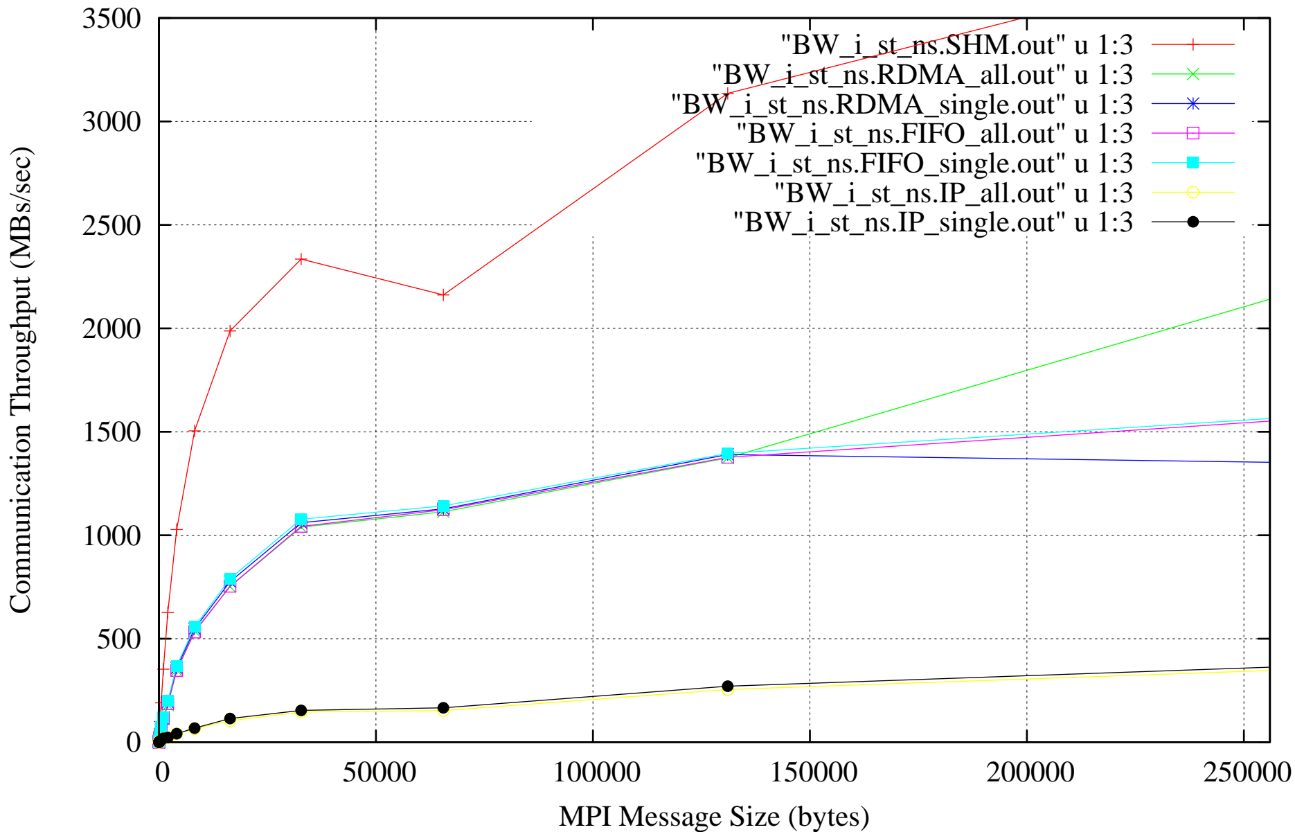
POE/MPI Communication Modes: Average (not_shared, blocking, interrupts, single-thread)
