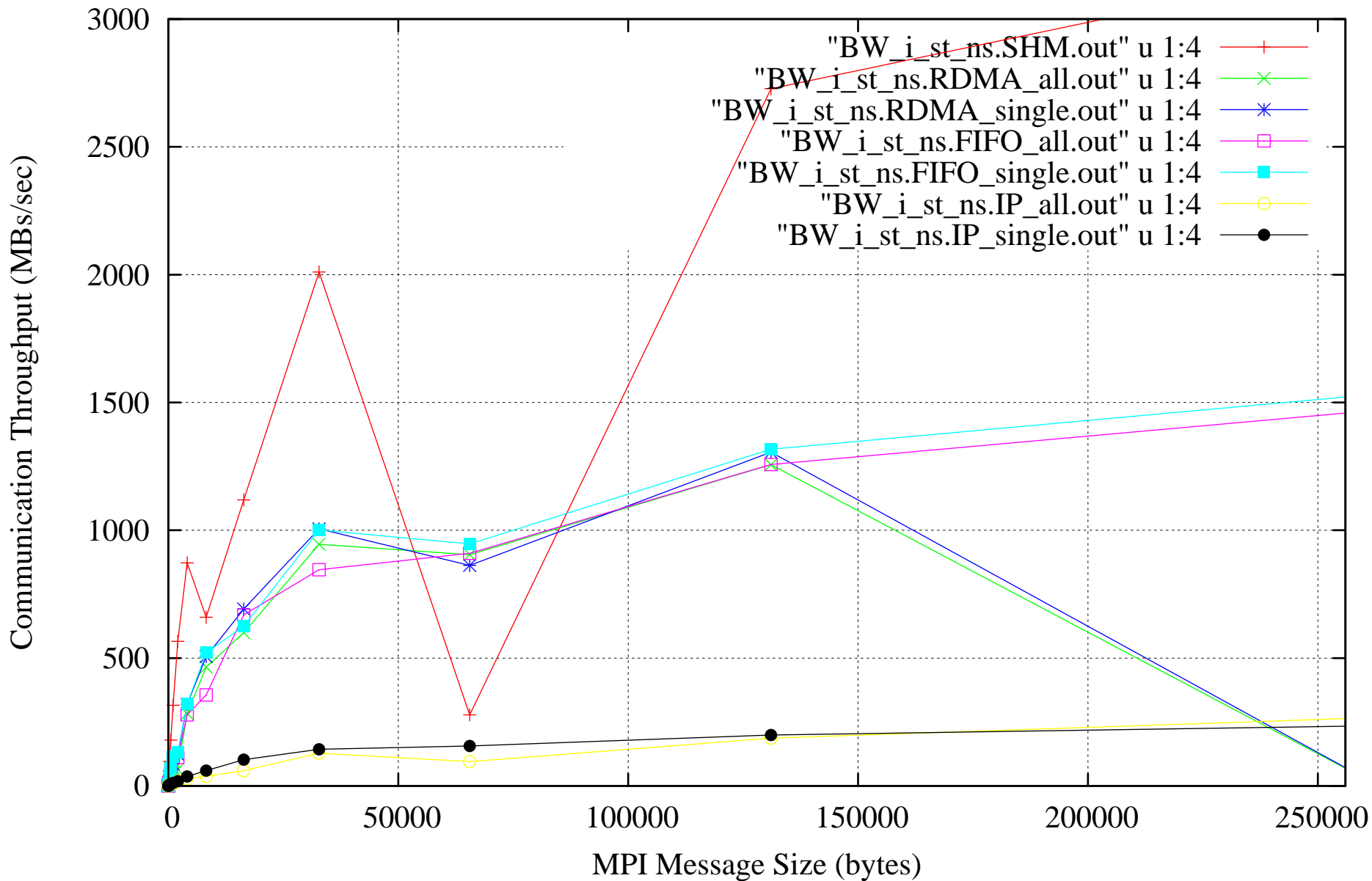
POE/MPI Communication Modes: Worst (not_shared, blocking, interrupts, single-thread)
