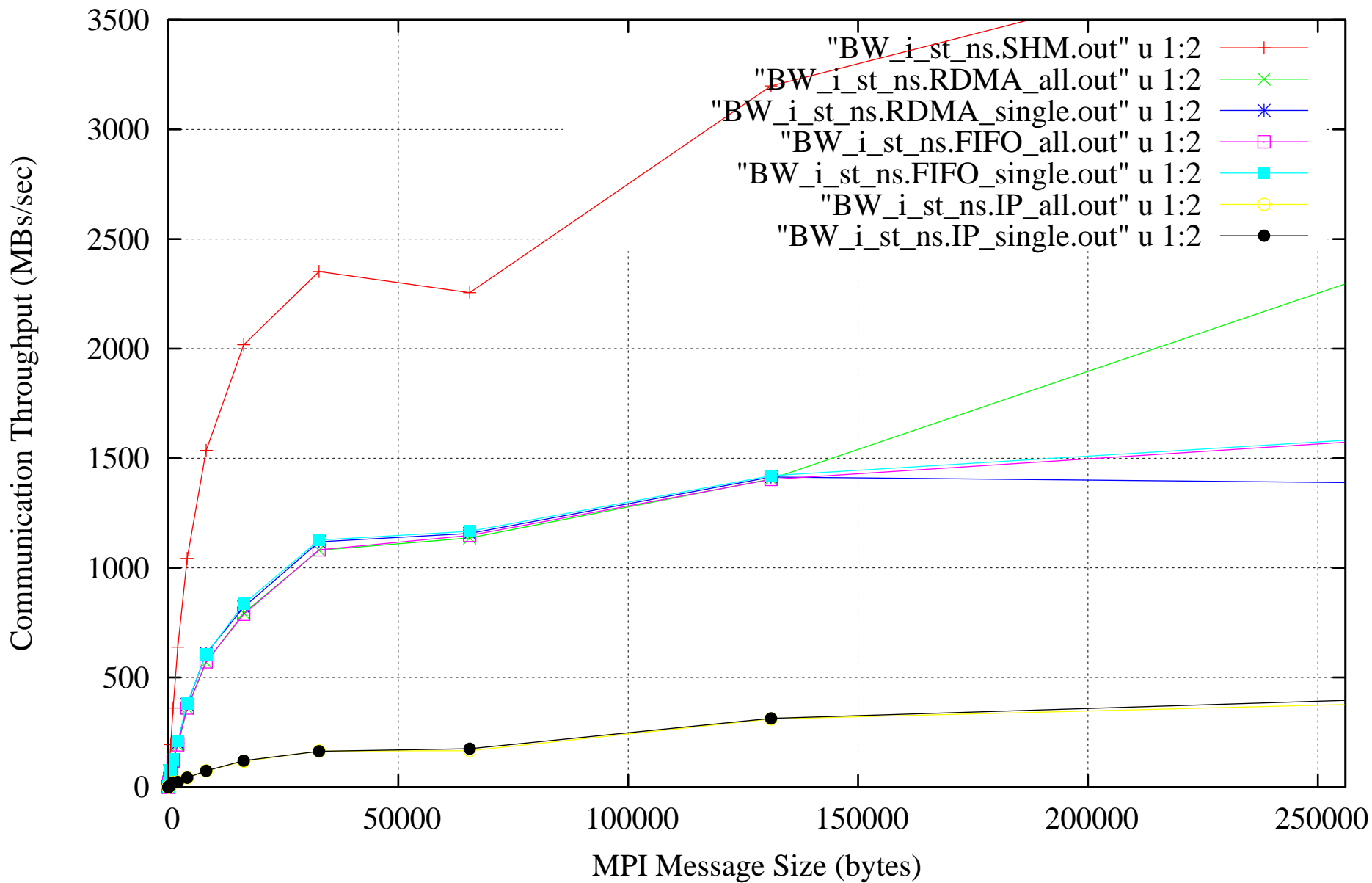
POE/MPI Communication Modes: Best (not_shared, blocking, interrupts, single-thread)
