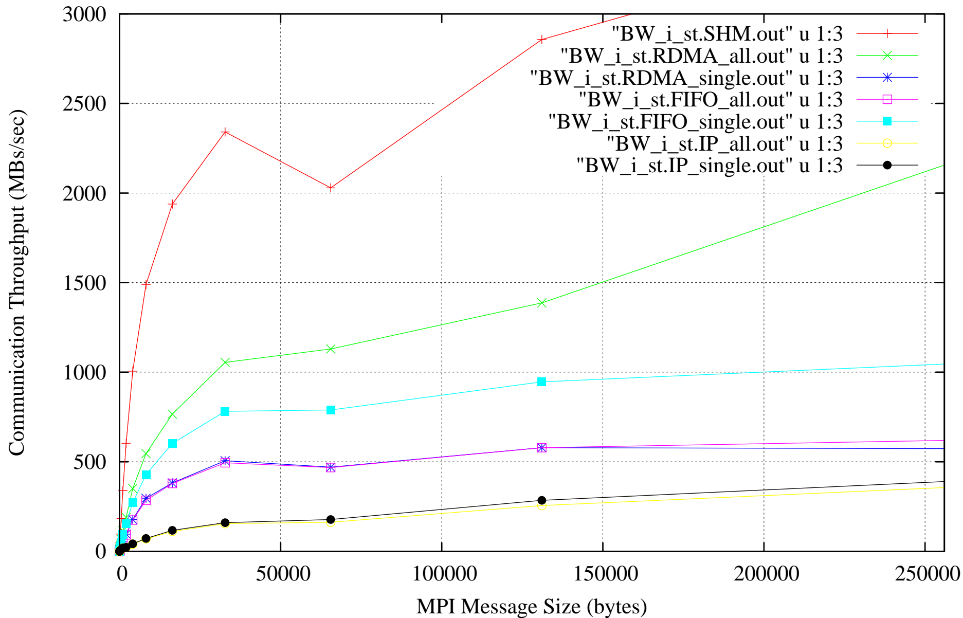
POE/MPI Communication Modes: Average (shared, blocking, interrupts, single-thread)
